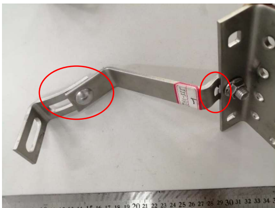
After test (2208013-1)
