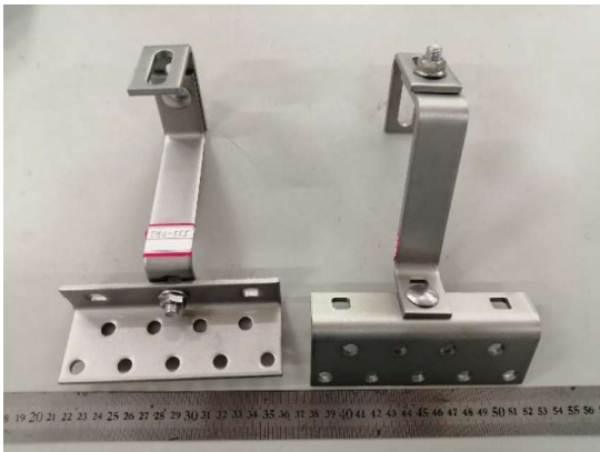
After test (2208013-1)
